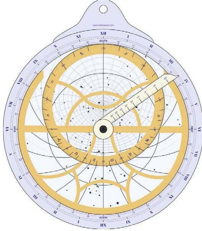
Figure 2: Schematic view of the projected star-map and reference circles of the astrolabe
